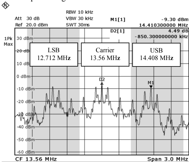
Figure 16: Measured ISO/IEC 14443 type A Manchester coded downlink spectrum of the active tag system
