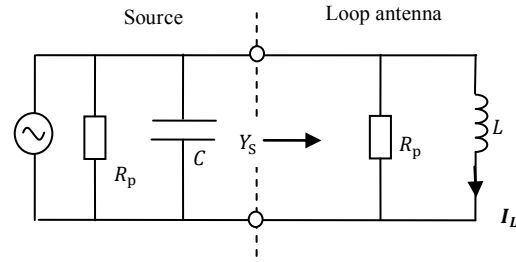
Figure 12: Active tag in transmitting mode (simplified configuration)
