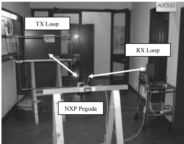
Figure 19: Measurement configuration in the lab corridor
