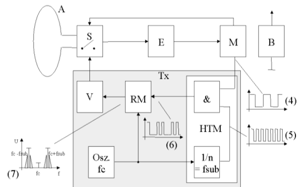
Figure 4: Basic circuit of a transponder, generating active load modulation.
