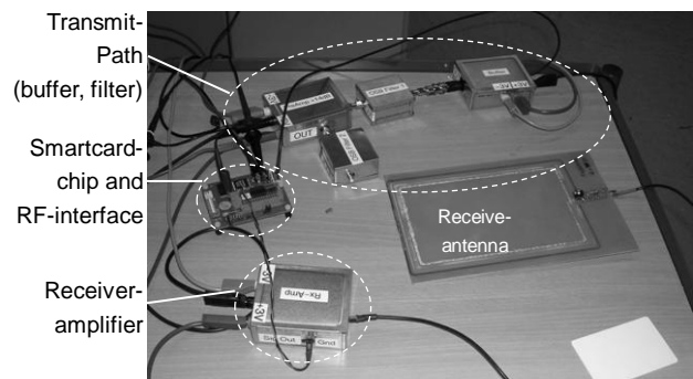
Figure 18: Discrete prototype implementation without TX-antenna
