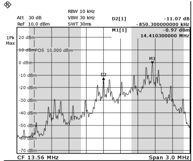
Figure 17: Measured ISO/IEC 14443 type A Manchester coded downlink spectrum of the active tag system after band pass filtering
