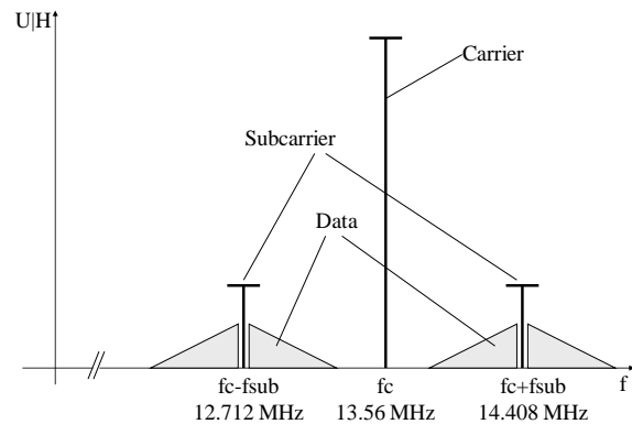
Figure 3 shows the frequency spectrum at the reader antenna resulting from load modulation with a subcarrier.
