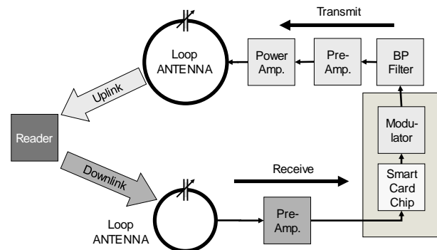
Figure 9: Prototype implementation
