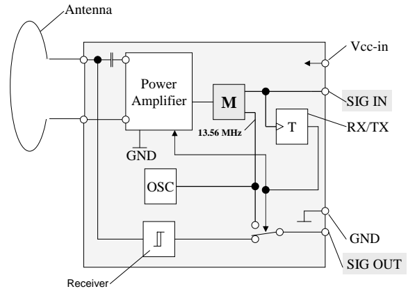
Figure 8 shows a simplified block diagram of the required active RFID interface module
