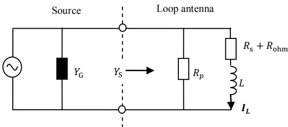
Figure 11: Active tag in transmitting mode
