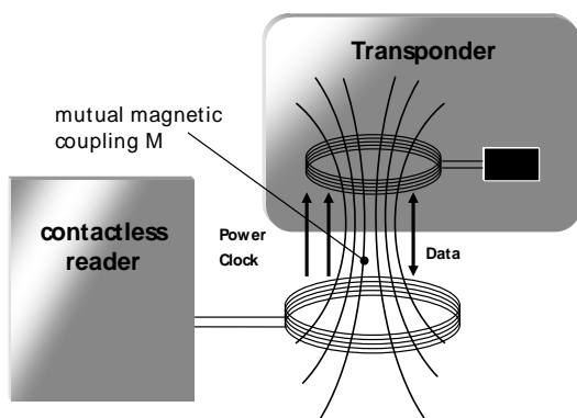
Figure 1: An inductively coupled RFID system uses mutual magnetic coupling to transfer power and data.
