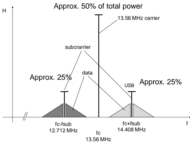
Figure 15: Power distribution of an ISO/IEC 14443 type A uplink signal
