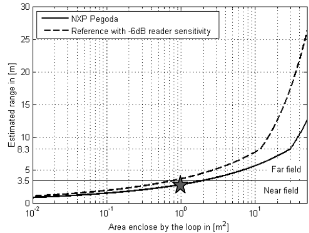
Figure 21: TX Antenna size extrapolation (star: measured range using a TX loop size of 1 \text{ m}^2 and a 50 Watt amplifier)
