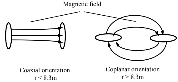
Figure 14: Optimum antenna orientation
