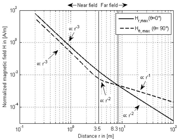
Figure 13: Normalized magnetic field of a small loop antenna in dependence of the distance (with a=1\text{m} and I_L=1\text{A} )
