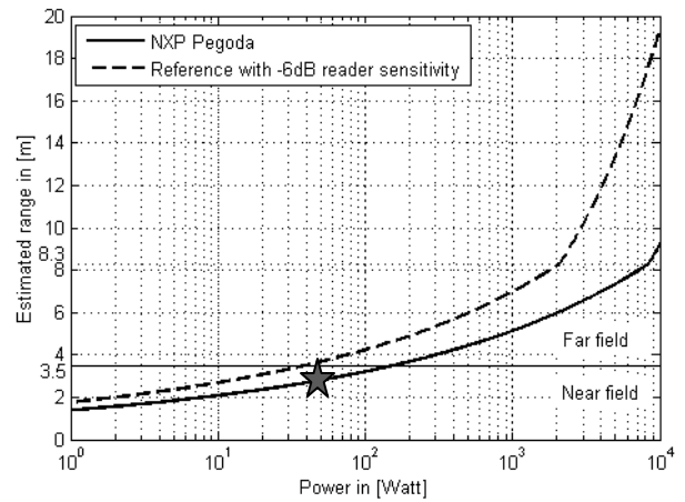
Figure 20: Power extrapolation (star: measured range using a TX loop size of 1 \text{ m}^2 and a 50 Watt amplifier)
