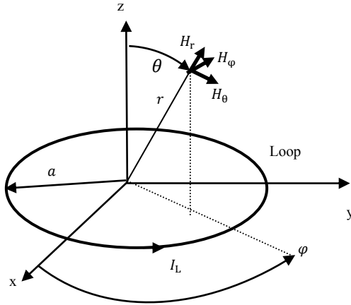
Figure 10: Coordinate system
